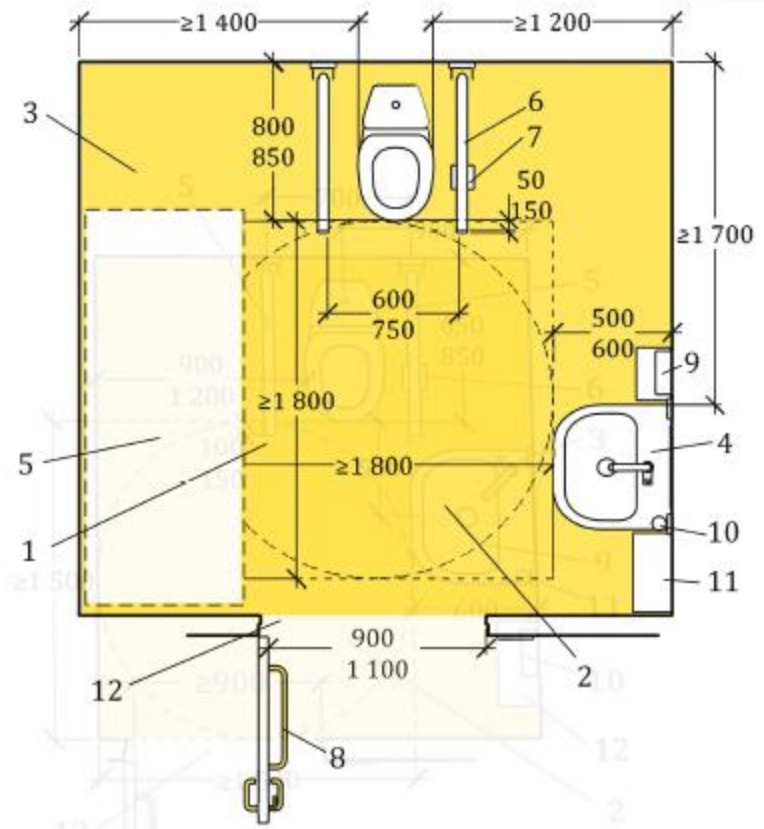
b) Large peninsular type toilet with bench and transfer space on both sides of pan
