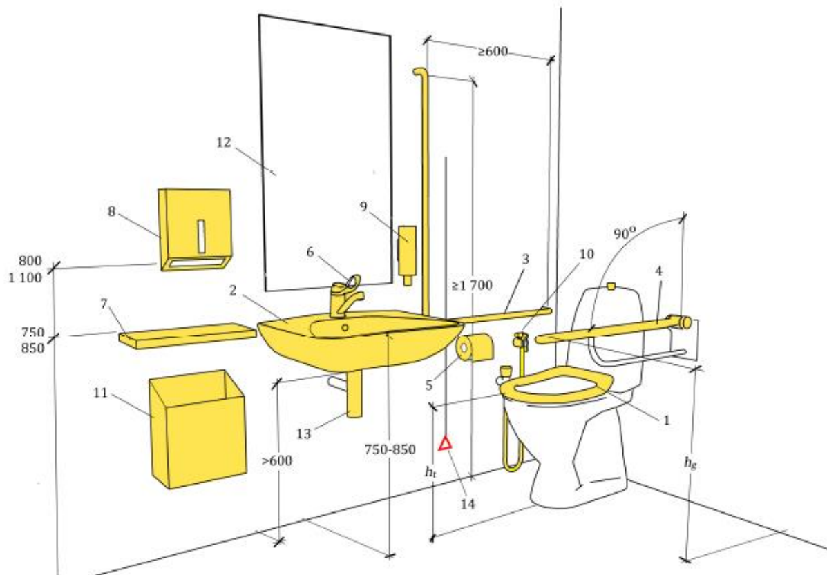
Figure 111 — Example of accessible toilet accessories
