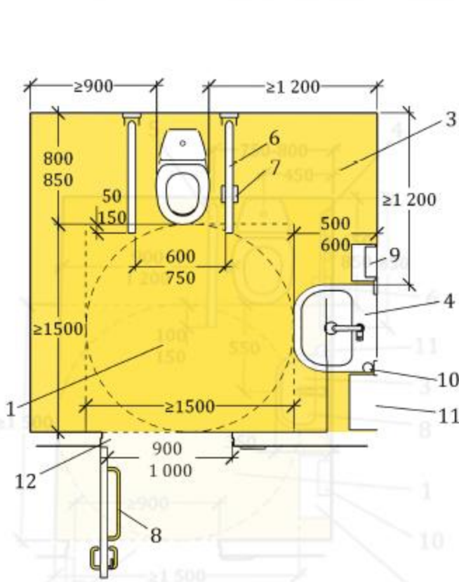
a) Peninsular type toilet with transfer space on both sides of pan
